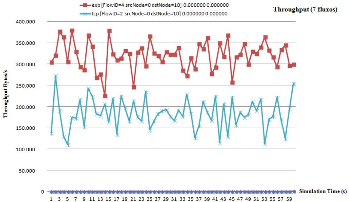
Figura 21: Throughput IPTV x TCP (7 fluxos)
