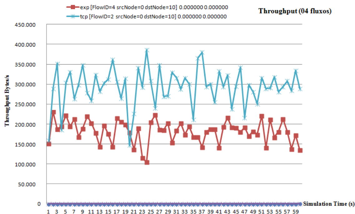
Figura 20: Throughput IPTV x TCP (4 fluxos)
