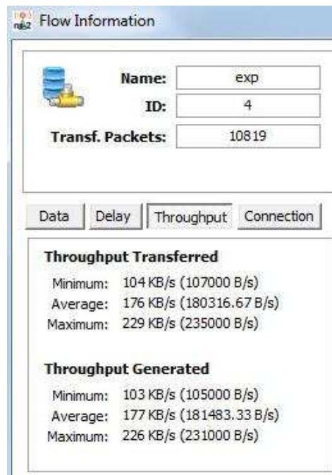
Figura 17: Throughput IPTV quatro fluxos
