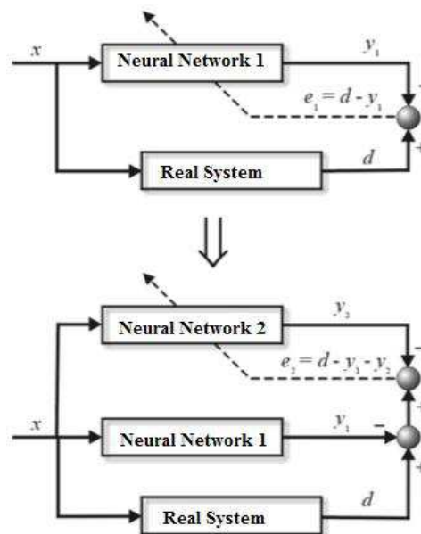
Figure 3. MNN arrangement with two networks.
