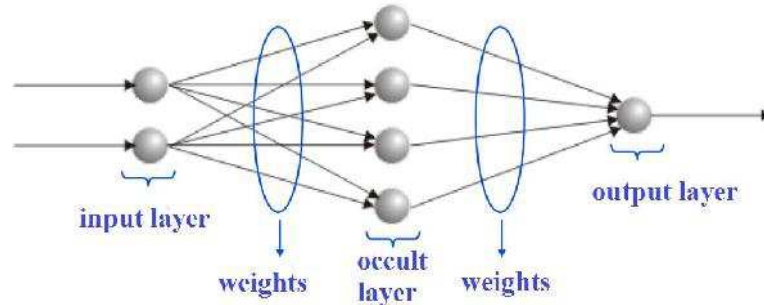
Figure 1. Structure of the ANN of MLP type
