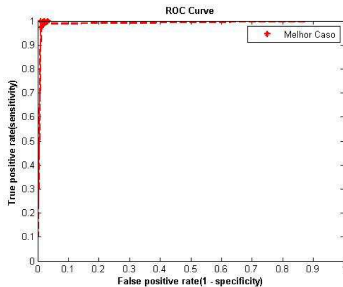
Figure 5. ROC Curve – Data base 1
