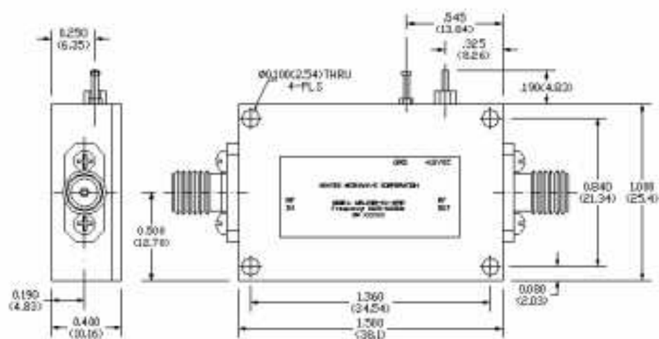
Mechanical Structure:
